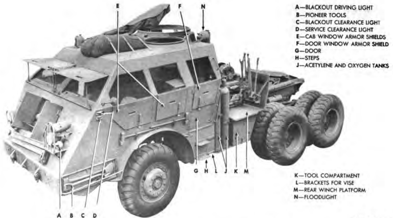
Figure 3—Left Front Three-quarter View of Tractor Truck M26 (Windows Open)
